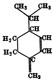
\beta -Phellandrene.
